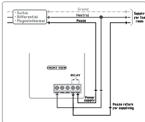
Standard Connecting Diagram:
