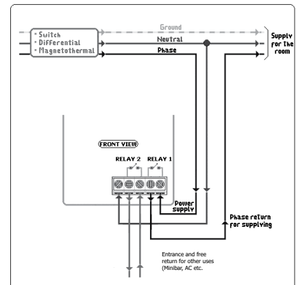
Intelligent Magnetic Stripe and RFID Connecting Diagram:
